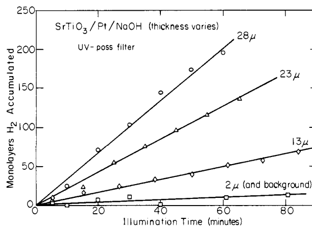
Figure 2. Hydrogen photoproduction from a platinized n-SrTiO 3 (111) crystal coated with NaOH to varying thicknesses, saturated with water vapor and illuminated through a Corning 7-51 filter.
