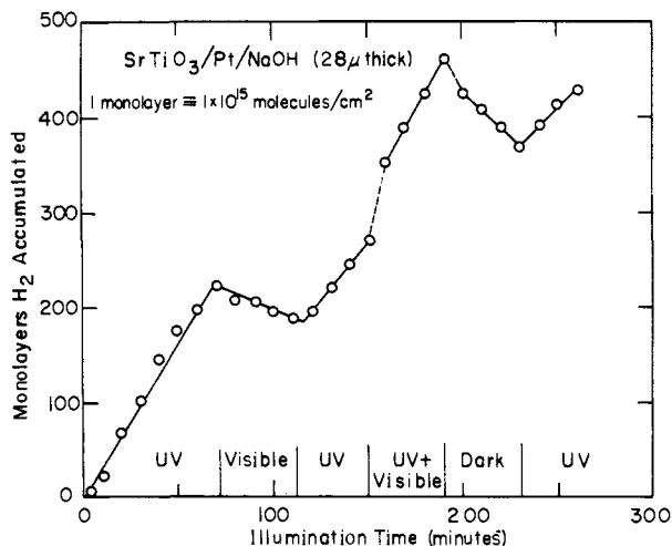
Figure 4. Coarse wavelength dependence of hydrogen photogeneration on a platinumized SrTiO 3 crystal coated with a 28- \mu m layer of NaOH and saturated with water vapor: light source, 500-W Hg lamp; "UV" = light passed by 2-cm H 2 O and a Corning 7-51 filter; "visible" = water and 3-74 filters; "UV + visible" = water filter only.
