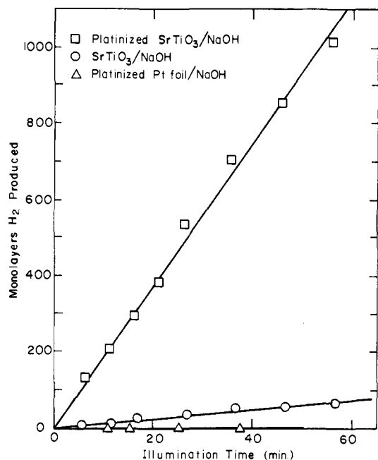
Figure 6. Comparison of hydrogen photoproduction from prereduced platinumized ( \square ) and metal-free ( \circ ) \text{SrTiO}_3 crystals and a platinumized platinum foil blank ( \triangle ). Each was supported in a Vycor glass holder, encrusted in NaOH, saturated with water vapor, and illuminated with the full output of the 500-W Hg lamp.
