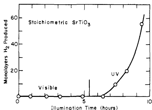
Figure 7. Hydrogen production from a stoichiometric, metal-free \text{SrTiO}_3(111) crystal in 19 N NaOH under visible (3-74 filter, 13 mW cm -2 ) and UV (7-51 filter, 4 mW cm -2 ) irradiation.
