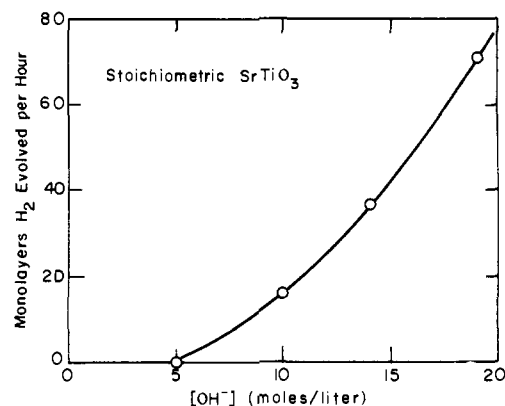
Figure 8. Hydrogen photoproduction at 44 °C on a stoichiometric, metal-free \text{SrTiO}_3(111) crystal as a function of electrolyte NaOH concentration. Illumination: full output of 500-W Hg lamp (23 mW cm -2 ).
