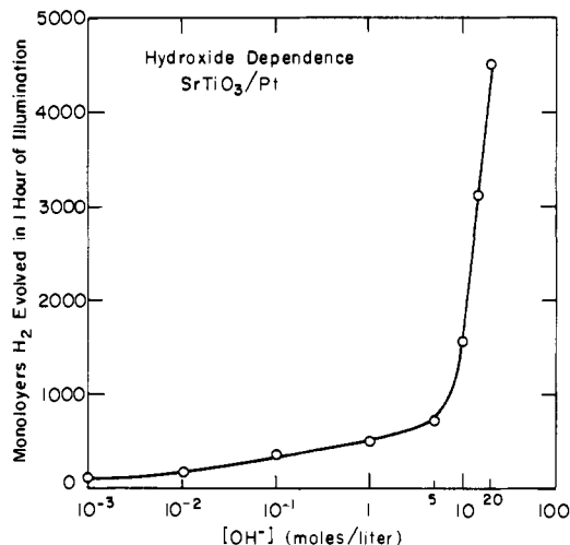
Figure 5. Rate of hydrogen photoproduction on a platinumized prerduced SrTiO 3 (111) crystal as a function of concentration of the aqueous NaOH electrolyte at 44 °C: light source, full output of 500-W Hg lamp; approximate scatter in data from other runs, \pm 35\% .
