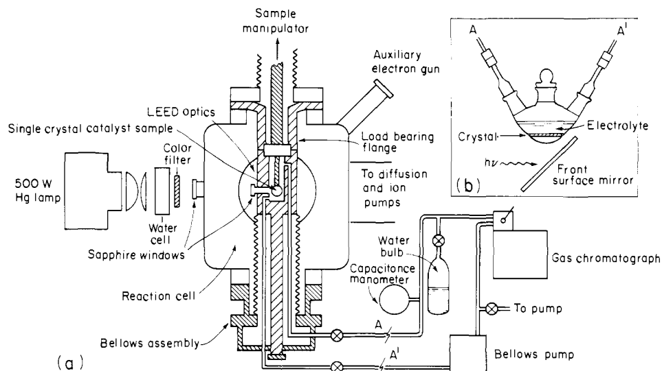
Figure 1. Experimental apparatus. (a) Closed circulation loop including gas-phase reaction cell within ultrahigh vacuum chamber. (b) Reaction cell for studies in bulk liquid electrolytes, which replaces the gas-phase reactor by attachment at points A and A'.
