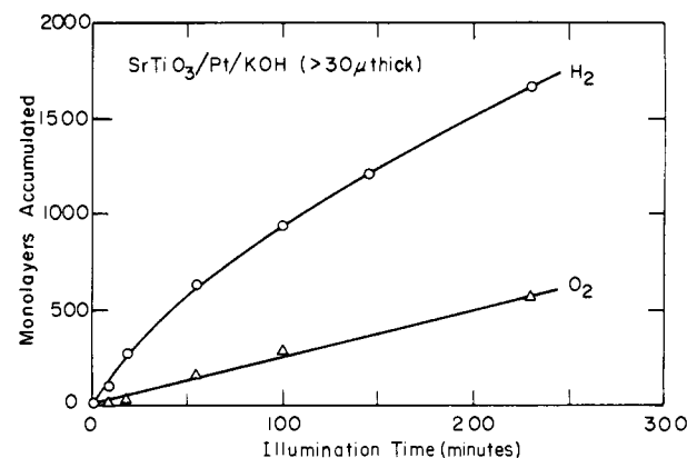
Figure 3. Hydrogen and oxygen photoproduction from a platinized n-SrTiO 3 crystal encrusted with KOH, saturated with water vapor, and illuminated with the full output of the 500-W Hg lamp.
